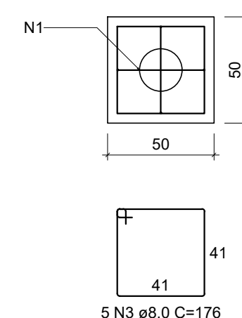
B4=B5=B8=B9=B10 1xC20 PLANTA ESC 1:25
