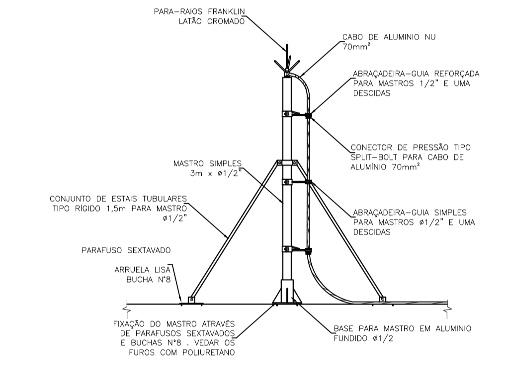
CAPTOR FRANKLIN COM MASTRO
